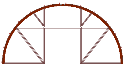
Braced end wall framing
