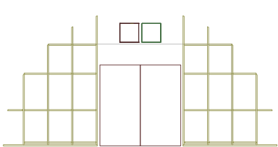
subframing and fixing rails
